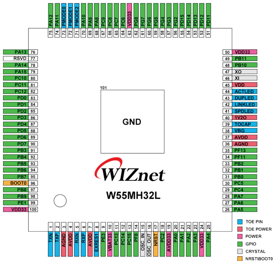
Figure 1 W55MH32L package
